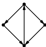
FIGURE 1. the directed graph G whose reflexive polytope cannot be obtained from any building set.
